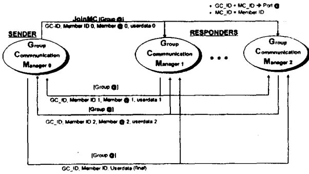
(Figure 4.3.d) Join MC procedure
