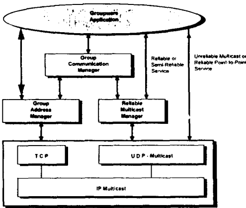
(Figure 4.1) Group Communication Management Architecture
