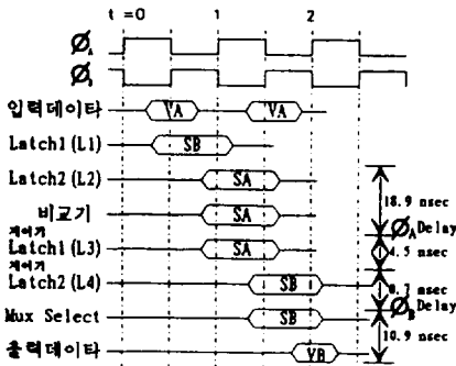
(b) Timing Analysis of Critical Path
