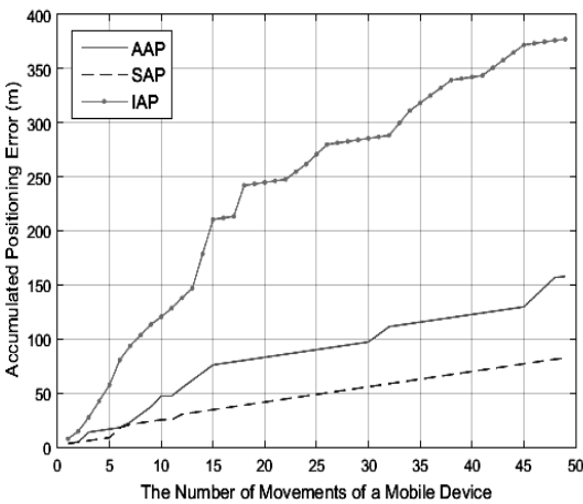
Fig. 7. An Accumulated Positioning Error (AAP vs. SAP vs. IAP)
