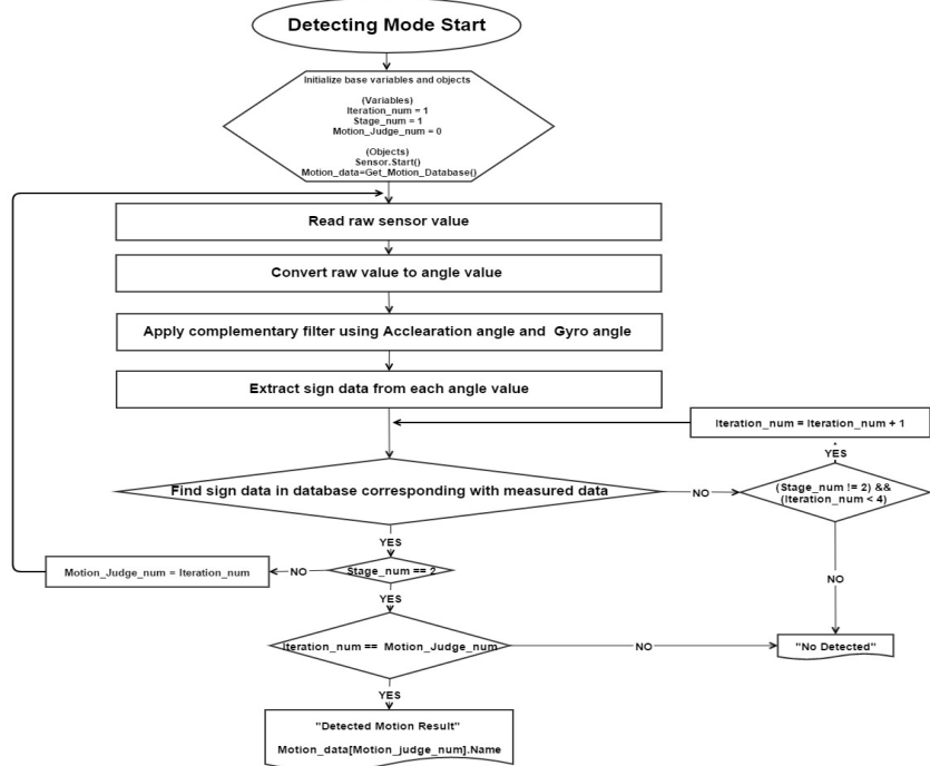
Fig. 14. Motion Detection Algorithm
