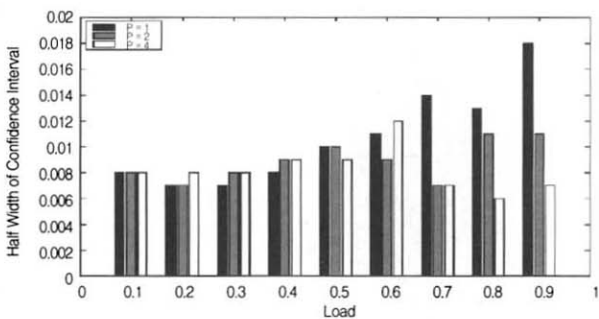
(Figure 11) Half-Width of Confidence Interval of Coverage Using 1, 2, and 4 Processors in Arcsin Transformation of M/D/1/\infty
