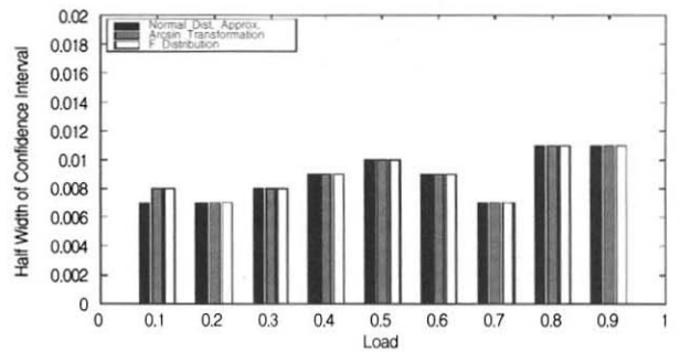
(Figure 5) Half-Width of Confidence Interval of Coverage Using Normal Distribution Approx., Arcsin Transformation and F-Distribution tApprox. in M/D/1/\infty ( P = 2 )
