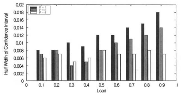
(Figure 7) Half-Width of Confidence Interval of Coverage Using 1, 2, and 4 Processors in Normal Distribution Approximation of M/M/1/\infty
