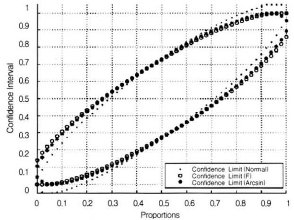
(Figure 13) Confidence intervals of proportions using normal, arcsin , and F distribution ( \alpha = 0.001 & n = 50 )
