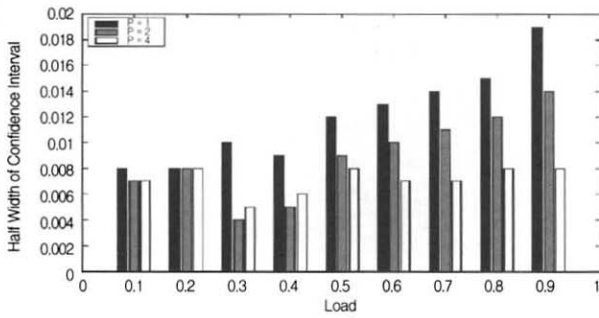
(Figure 9) Half-Width of Confidence Interval of Coverage Using 1, 2, and 4 Processors in F -Distribution Approximation of M/M/1/\infty
