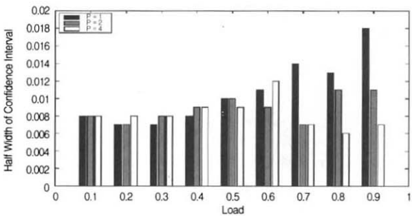
(Figure 12) Half-Width of Confidence Interval of Coverage Using 1, 2, and 4 Processors in F -Distribution Approximation of M/D/1/\infty
