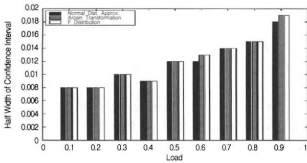
(Figure 1) Half-Width of Confidence Interval of Coverage Using Normal Distribution Approx., Arcsin Transformation and F-Distribution Approx. in M/M/1/\infty ( P = 1 )
