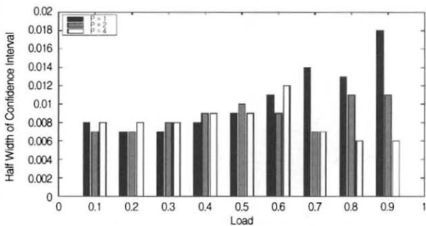
(Figure 10) Half-Width of Confidence Interval of Coverage Using 1, 2, and 4 Processors in Normal Distribution Approximation of M/D/1/\infty
