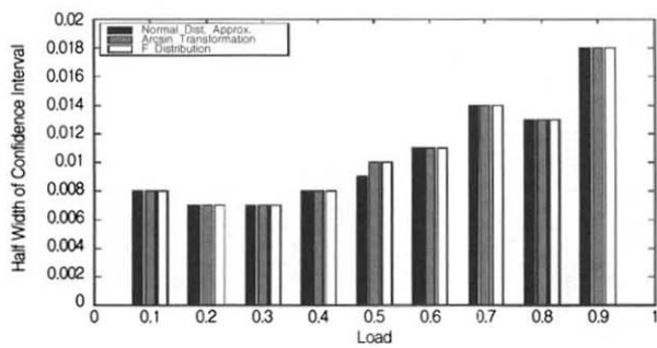
(Figure 4) Half-Width of Confidence Interval of Coverage Using Normal Distribution Approx., Arcsin Transformation and F-Distribution Approx. in M/D/1/\infty ( P = 1 )
