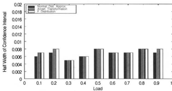
(Figure 3) Half-Width of Confidence Interval of Coverage Using Normal Distribution Approx., Arcsin Transformation and F-Distribution Approx. in M/M/1/\infty ( P = 4 )
