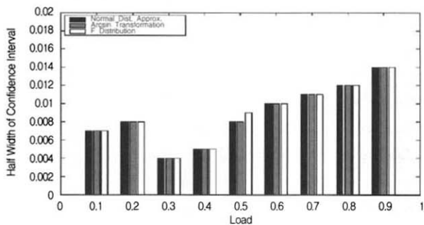
(Figure 2) Half-Width of Confidence Interval of Coverage Using Normal Distribution Approx., Arcsin Transformation and F-Distribution Approx. in M/M/1/\infty ( P = 2 )
