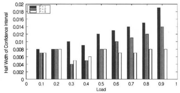
(Figure 8) Half-Width of Confidence Interval of Coverage Using 1, 2, and 4 Processors in Arcsin Transformation of M/M/1/\infty
