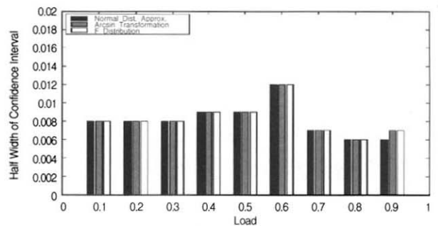
(Figure 6) Half-Width of Confidence Interval of Coverage Using Normal Distribution Approx., Arcsin Transformation and F-Distribution Approx. in M/D/1/\infty ( P = 4 )
