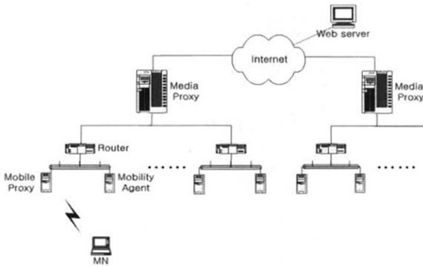
(그림 1) Two-tiered proxy system architecture
