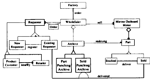
(b) Object Model for Wholesale Application
