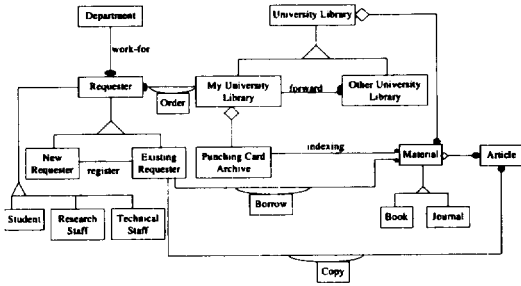
(a) Object Model for Library Application
