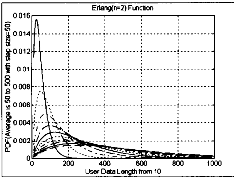
(a) Erlang 함수 분포 (a) Erlang distribution
