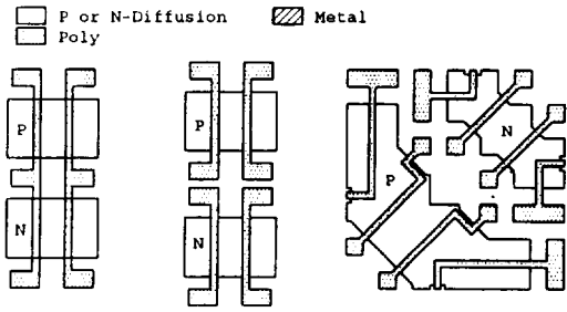
(a) Oxide-isolation 구조 [1, 5, 11].
