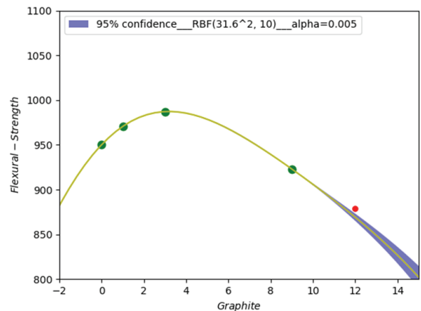
Fig. 7. Graphite vs Flexural-Strength = f1(x)
