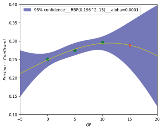
Fig. 10. GF vs Friction-Coeff = g_2(x)
