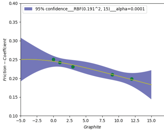
Fig. 8. Graphite vs Friction-Coeff = g_1(x)
