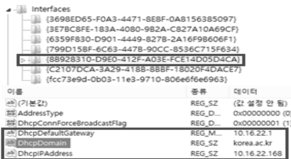
Fig. 14. Assigned IP Address Information
