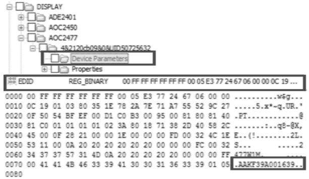
Fig. 2. The Serial Number of the Monitor
