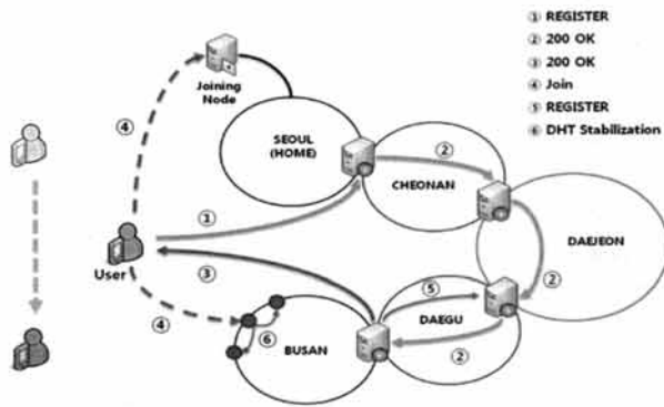
Fig. 6. Registration Mechanism
