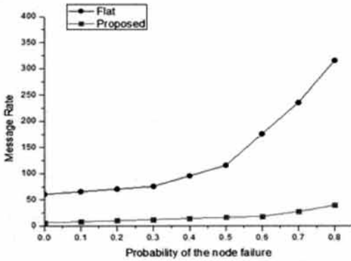
Fig. 11. Message rates (probability of the node failure)
