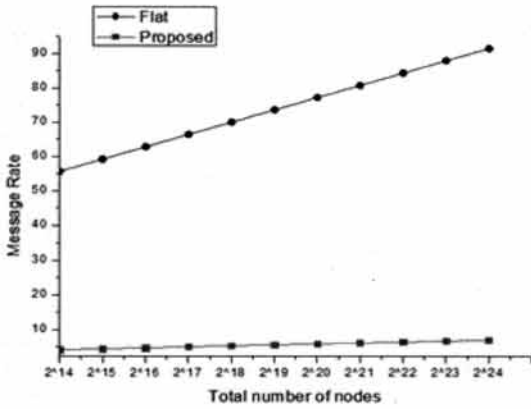
Fig. 10. Message rates (total numbers of nodes)
