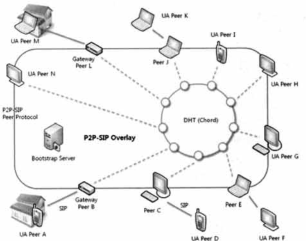
Fig. 2. P2P-SIP Architecture
