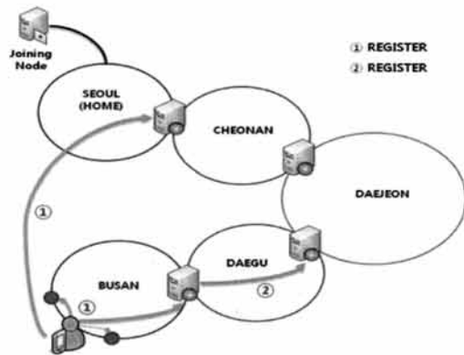
Fig. 7. Move Mechanism
