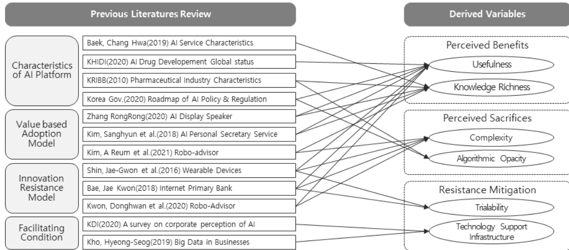
Fig. 1. Derivation of Research Variables
