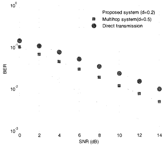
(Fig. 5) BER performance of transmission protocols
