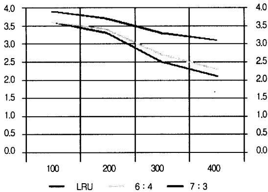
(Figure 4) Mean value of response time (sec.) : compare with LRU
