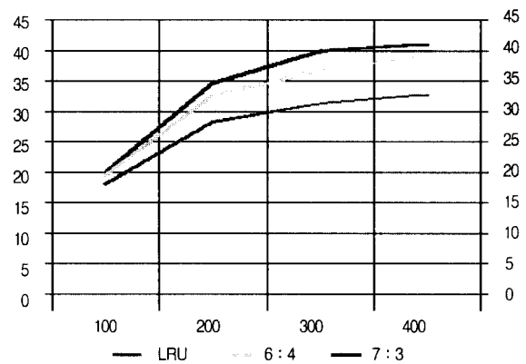
(Figure 2) Mean value of object hit ratio (%) : compare with LRU
