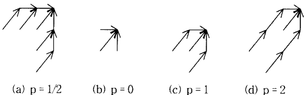
(Figure 2) DTW slope constraint
