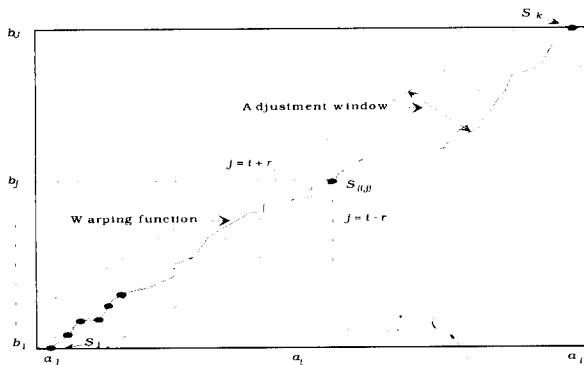
(Figure 1) DTW mechanism for time alignment
