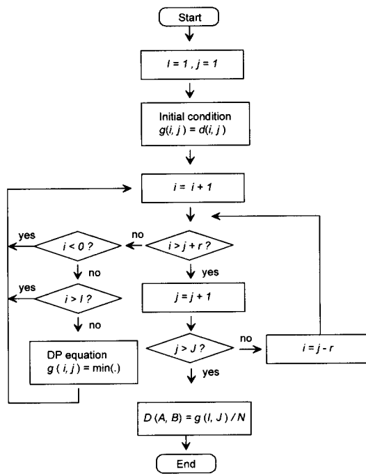
(Figure 3) DTW implementation
