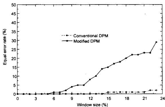
(Figure 10) Group I MDPM result
