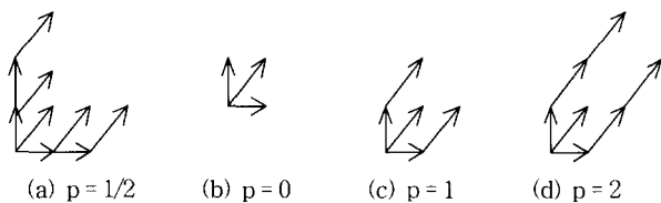
(Figure 8) MDTW slope constraint
